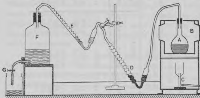
Fig. 1. Hydrogen sulphide determination. A. Fermentation flask; B. incubator; C. regulated warming; D. globe-tube with iodine solution; E. globe-tube with Natr. thiosulphate solution; F. aspirator.
