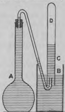
Fig. 2. Anaerobic decomposition of cellulose. A. Fermentation flask; B. water container; C. gas measuring tube; D. gaseous products.
